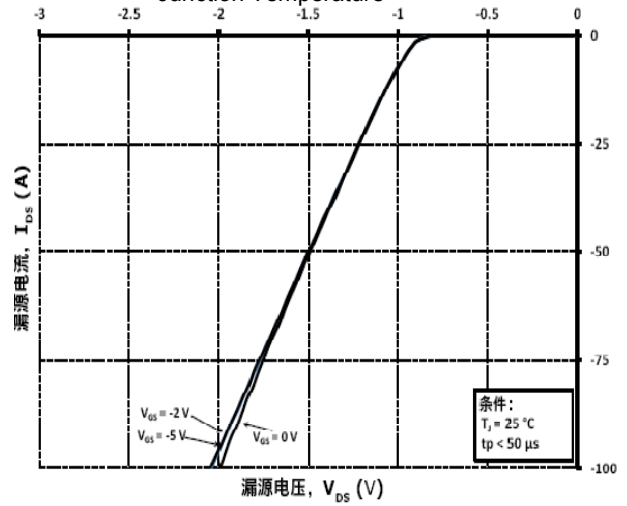
Fig.10 Diode Characteristic at 25°C
