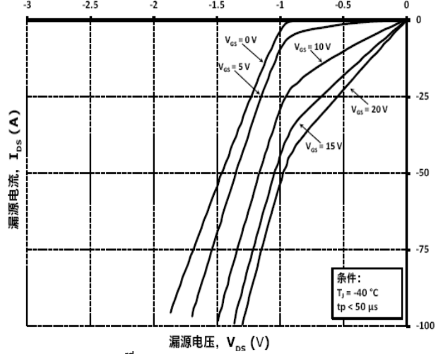
Fig.12 3 rd Quadrant Characteristic at -40°C
